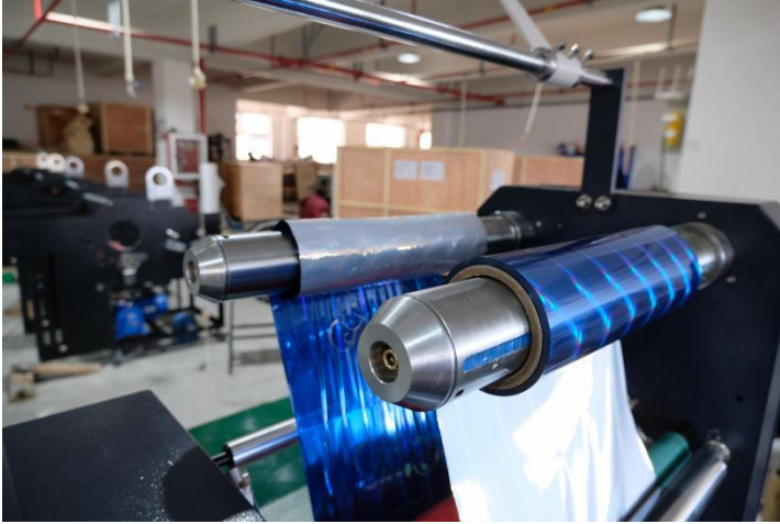
FOIL REWINDING AIR SHAFT
