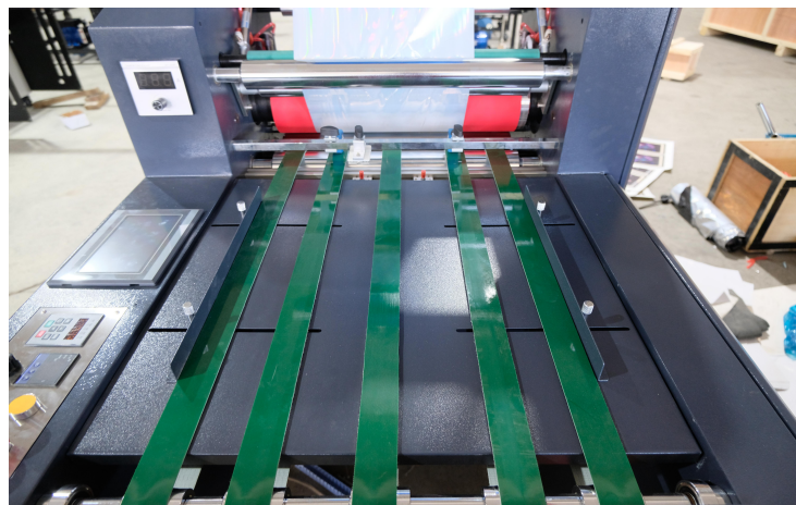
PAPER FEEDING TABLE
